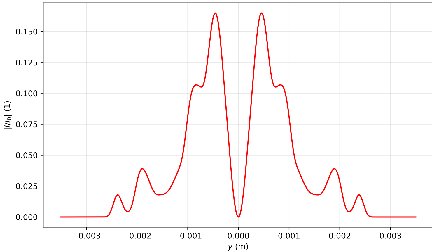
Intensity profile I(x=0, y, z=3.184)/I_0 , \text{Pin}=9.0\text{Pcr} , artificial time
